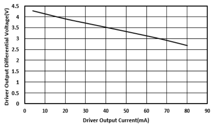
Figure 7-2 Driver Differential Output Voltage vs Driver Output Current
