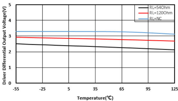
Figure 7-5 Driver Differential Output Voltage vs. Temperature
