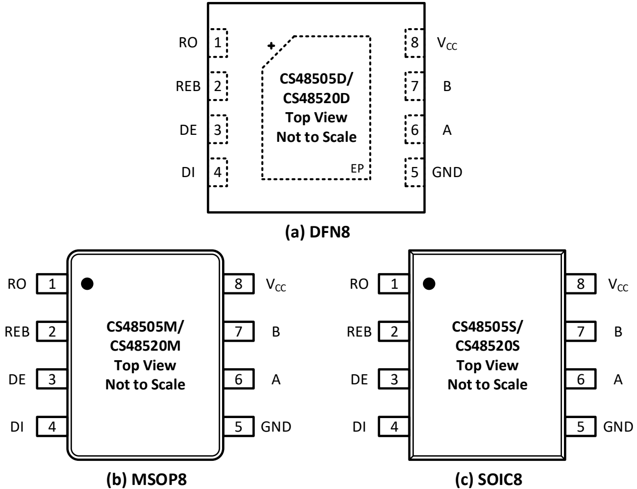
Figure 6-1. CS485xx pin configuration
