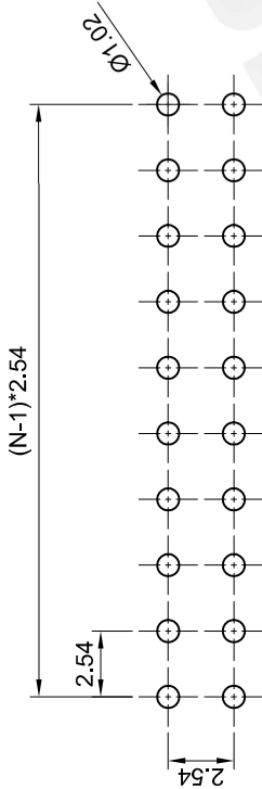
Recommend PCB Layout
