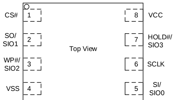
Figure 2-1. Connect Diagram
