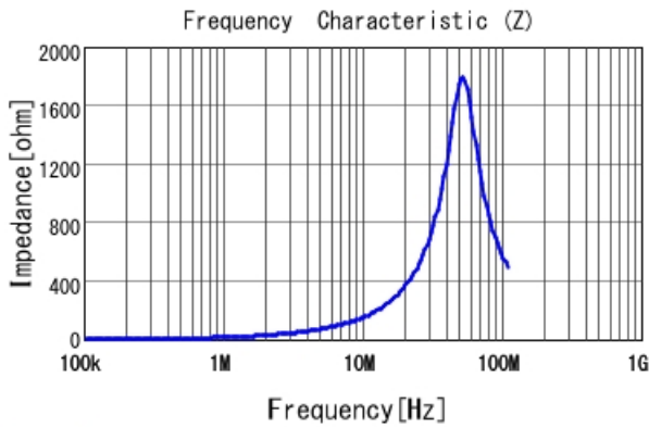
LQM2HPN2R2MG0 |Z|
