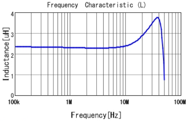
LQM2HPN2R2MG0 L
