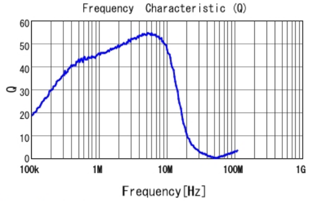
LQM2HPN2R2MG0 Q
