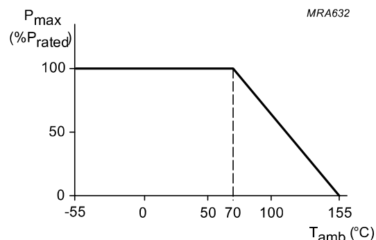
Fig. 10-1 Maximum dissipation (P) in percentage of rated power as a function of the operating ambient temperature (T amb )
