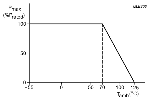
Fig. 10-2 Maximum dissipation (P) in percentage of rated power as a function of the operating ambient temperature (T amb )
